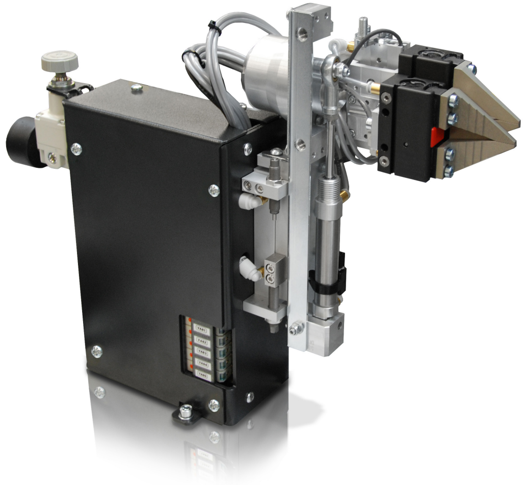
SLD 4100 Double Gripper Module for CrimpCenter
